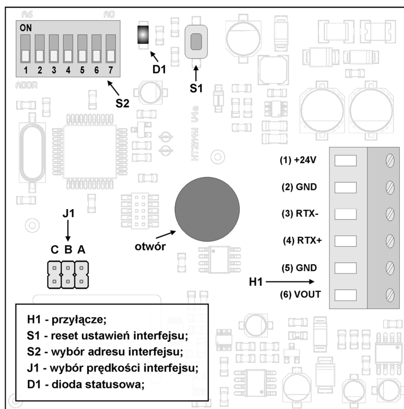
Figure 2. Transducer terminal description in a wall version .
