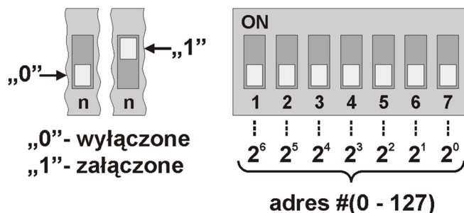
Figure 4. Transducer addressing.
