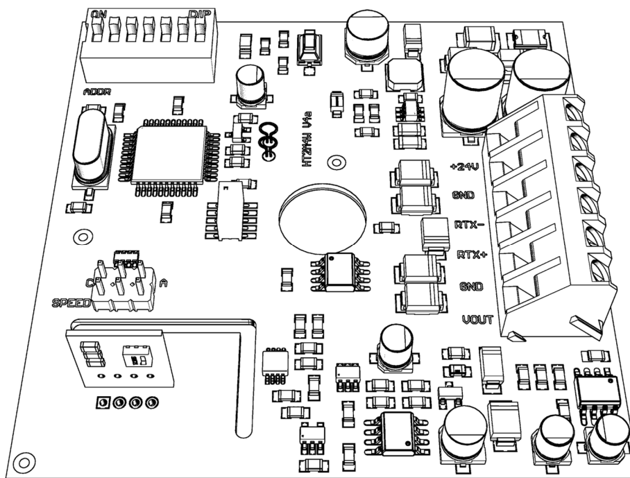
Figure 1. View of the circuit of the printed version of the wall transducer.
