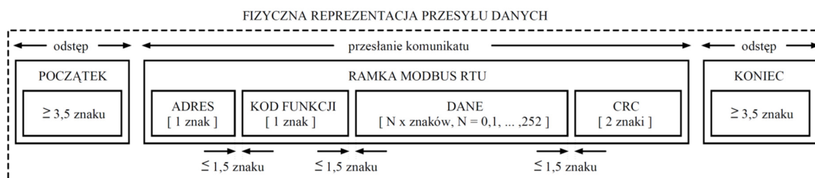
Figure 7. Data transfer in the MODBUS RTU standard implemented in the transducer.
