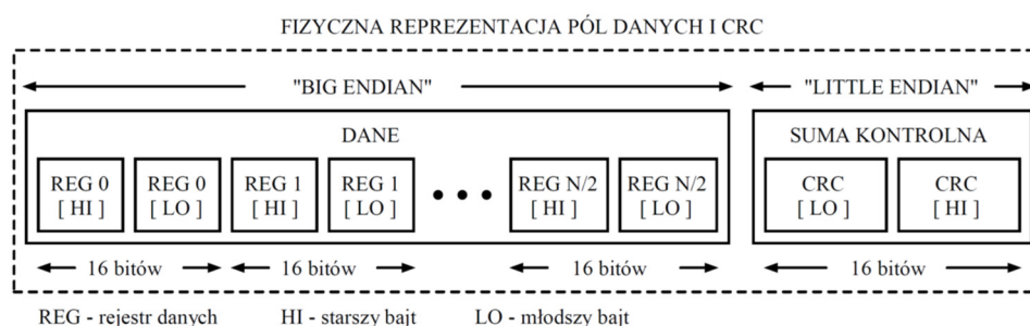
Figure 9. Format of data fields and CRC in the MODBUS RTU standard used in the transducer.
