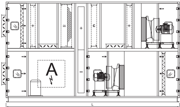
PVS PO dehumidification unit with preheater
