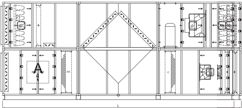
PVS PCR dehumidification unit with preheater
