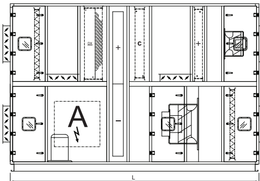
PVS PO dehumidification unit without preheater
