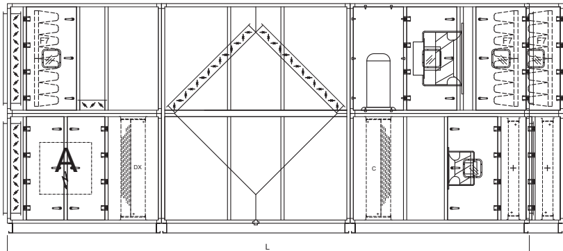
PVS PCR dehumidification unit without preheater
