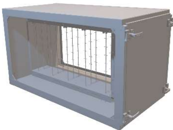
Figure 2 - electric heater in the AHU casing
