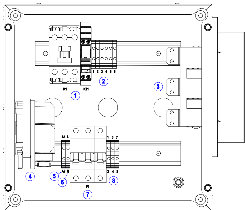
Figure 4 – power box – type 1x18kW
