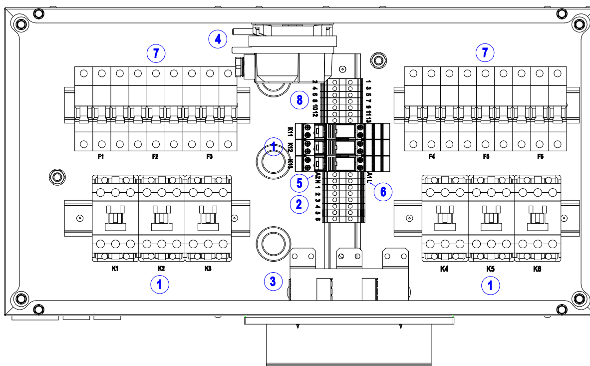
Figure 5 – power box – type 6x18kW
