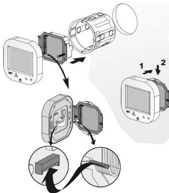
Assembly diagram
