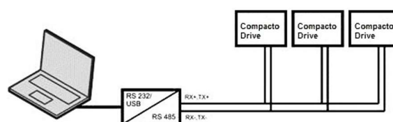
Parallel connections
